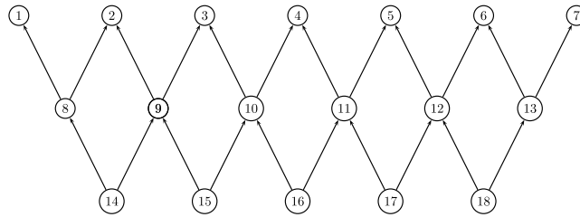
Fig. 1. Example PCKP: a_i = 1, i = 1, \dots, 18, b = 10 , note that C = \{15, 16, 17\} is a MIC, but not a facet for the problem. In particular, x_3, x_4, x_5 must be one whenever x_{15} + x_{16} + x_{17} = 2 .
